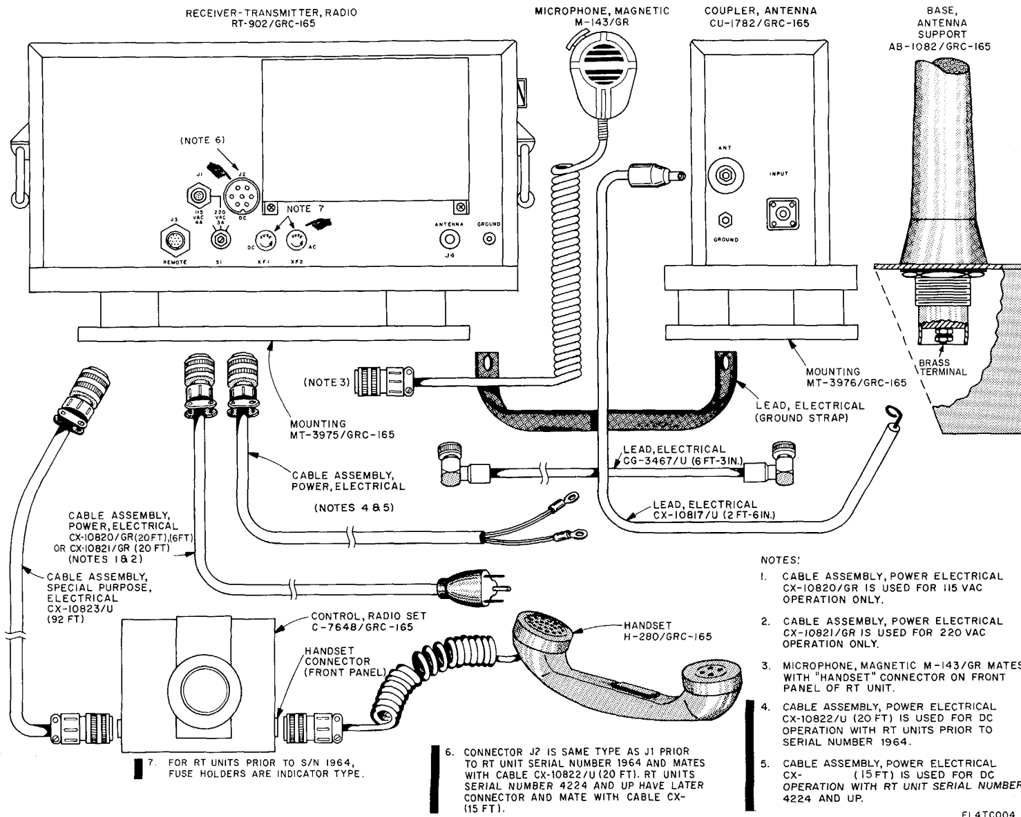
Figure 2-2. Radio Set AN/GRC-165 and Control, Radio Set C-7648/GRC-165 pictorial cabling diagram.
