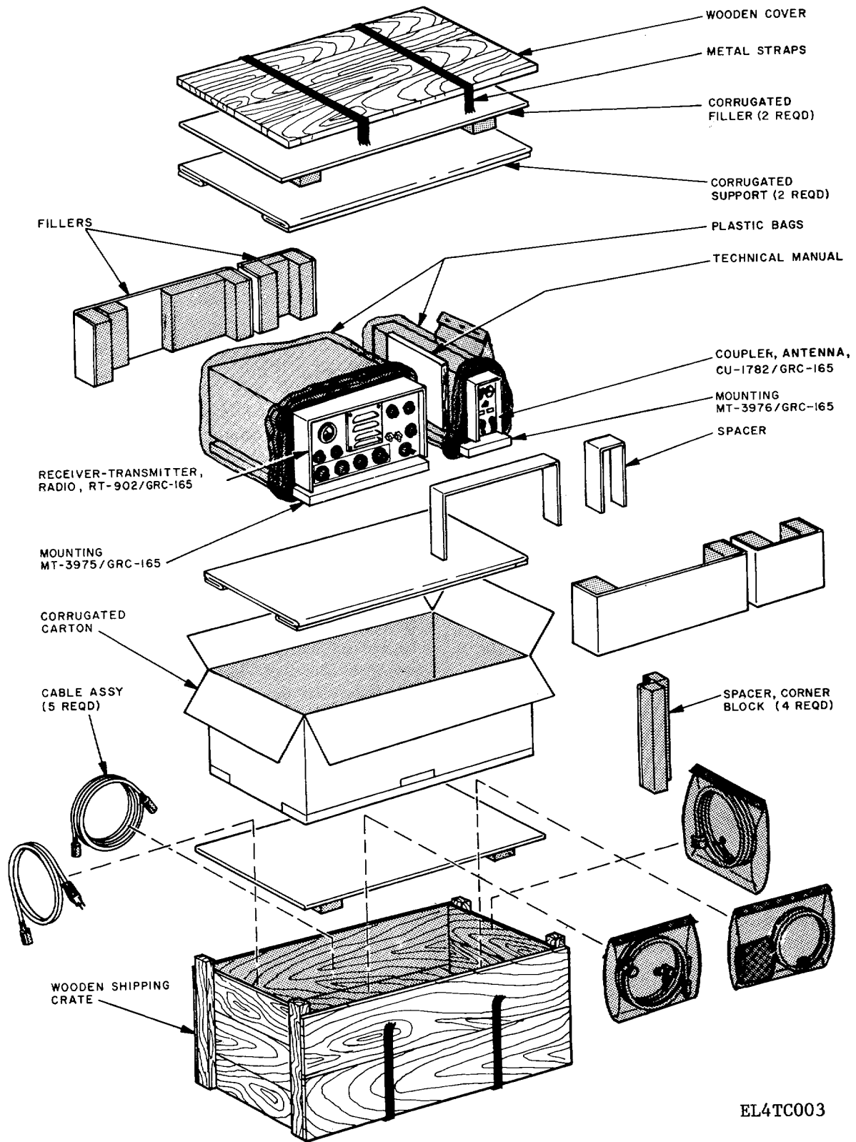
Figure 2-1. Typical packaging.
